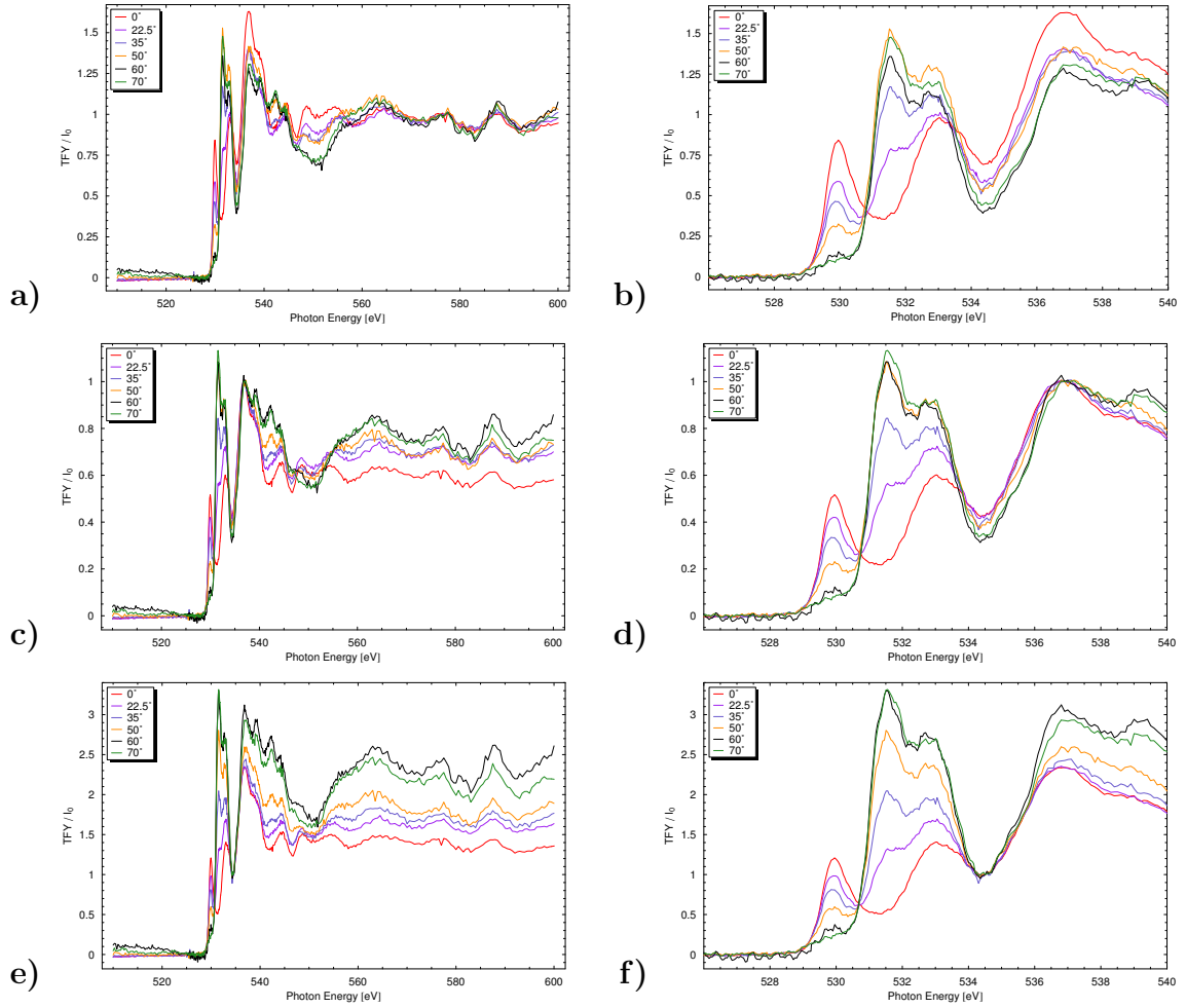
Figure B.2: Evolution of oxygen K edge with angle for T_c = 9.5 K Tl-2201 crystal, normalized several different ways. Panels a) , c) and e) are normalized well above the edge, on the edge, and in the notch between the prepeaks and edge respectively, while panels b) , d) and f) show the prepeak and oxygen K edge in more detail for each respective spectrum.
