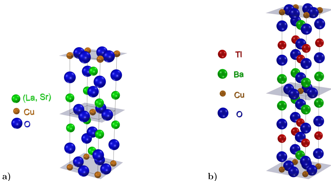
Figure 1.3: Unit cells of the high-temperature superconductors a) LSCO and b) Tl-2201. Copper oxide planes are emphasized through the use of shading. Each compound is body-centred, and thus has two copper oxide planes per unit cell in identical chemical environments.
