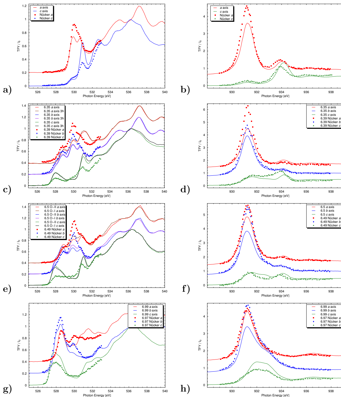
Figure A.16: Polarization dependence of each edge, compared against Nücker's results [85]: a) and b) show 7 - \delta = 6.0 , c) and d) 6.35, e) and f) 6.5, and g) and h) the 6.99 spectra. Panels a) , c) , e) , and g) present the O K edge results, while panels b) , d) , f) , and h) show the Cu L edge.
