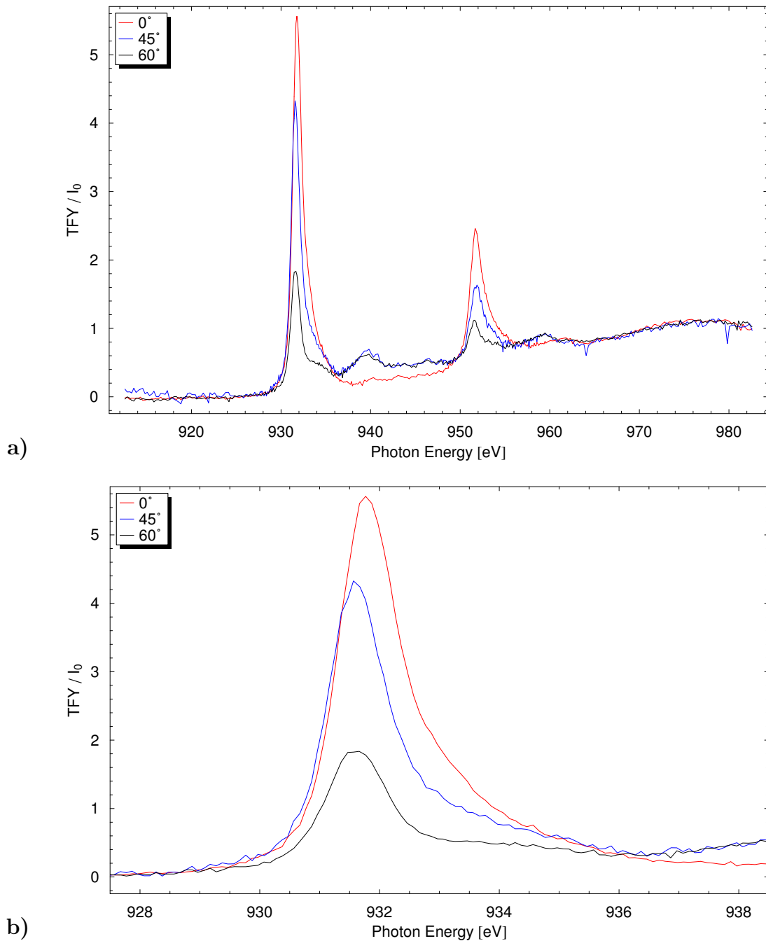
Figure B.10: Evolution of Cu L edge with angle for T_c = 69 K Tl-2201 crystal. a) Entire spectrum for all angles, and b) detail of the Cu L\alpha peak. These scans originally had backgrounds that prevented them from being effectively compared. A parabola was fit to the difference between each higher-angle scan and the 0^\circ scan (well away from the edges) and subtracted.
