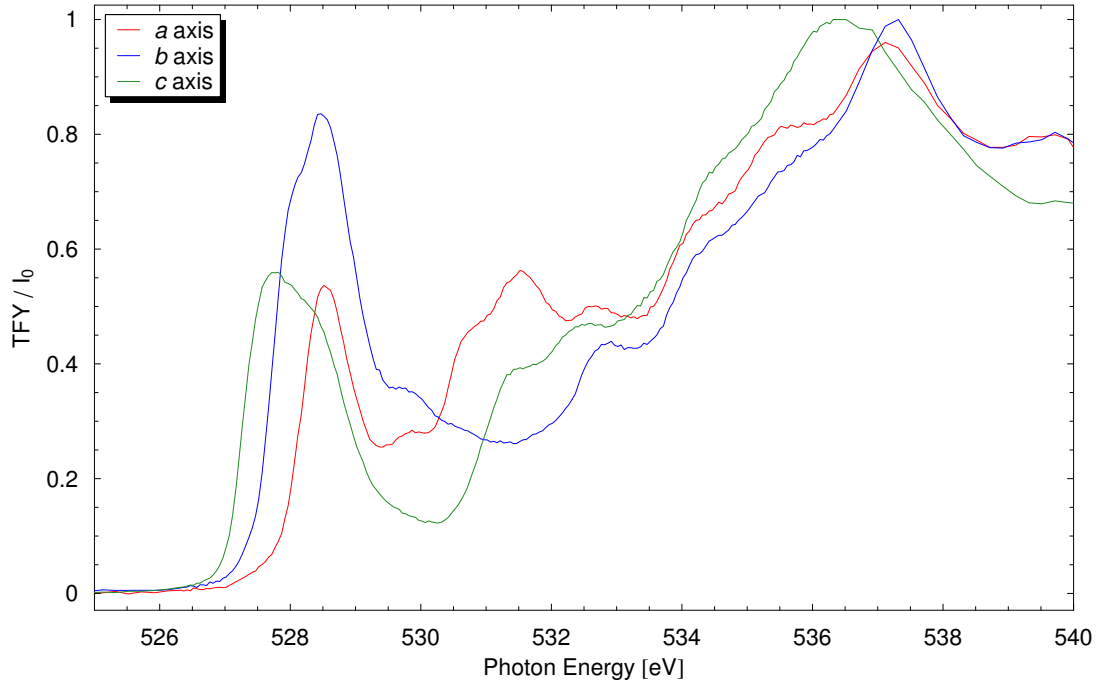
Figure 4.4: Oxygen K edge for \text{YBa}_2\text{Cu}_3\text{O}_{6.99} as a function of polarization.
