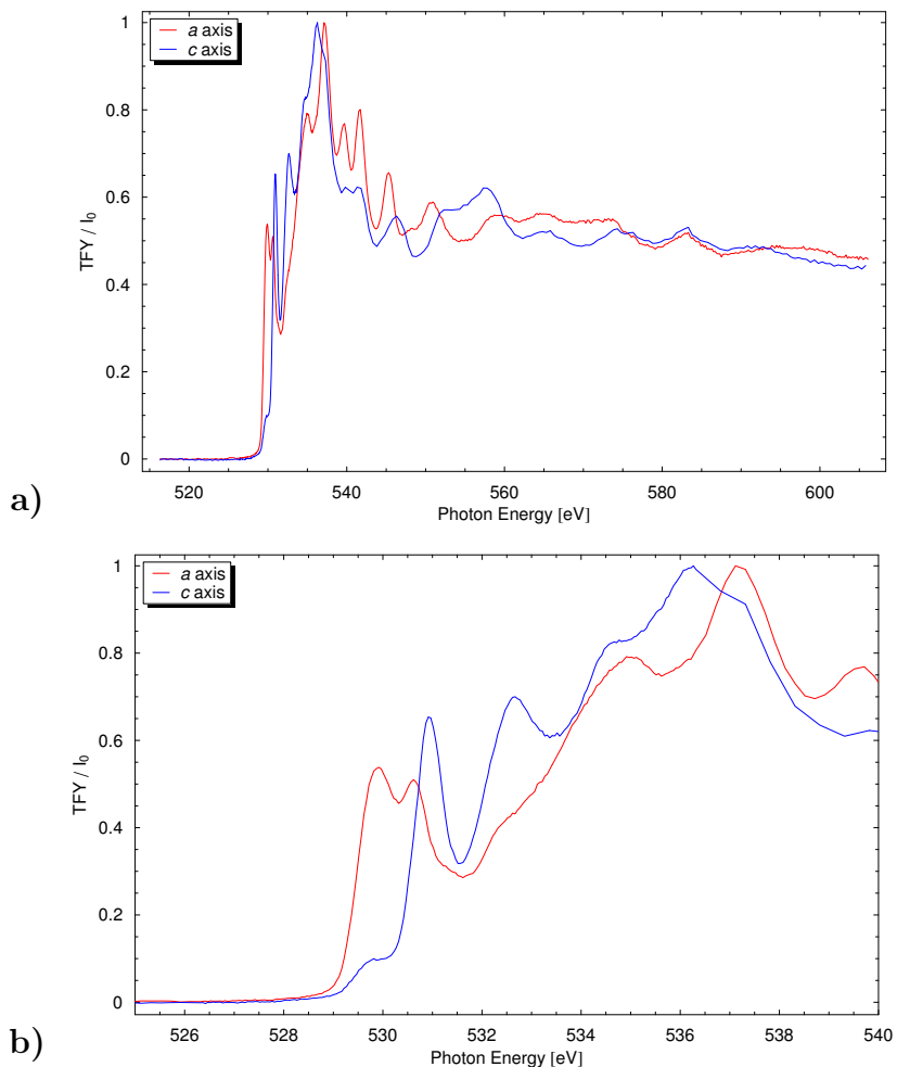
Figure A.2: Oxygen K edge for YBa 2 Cu 3 O 6.0 : a) Entire spectrum, and b) detail of the O K edge and prepeaks. Recall that the b axis is identical to the a axis.
