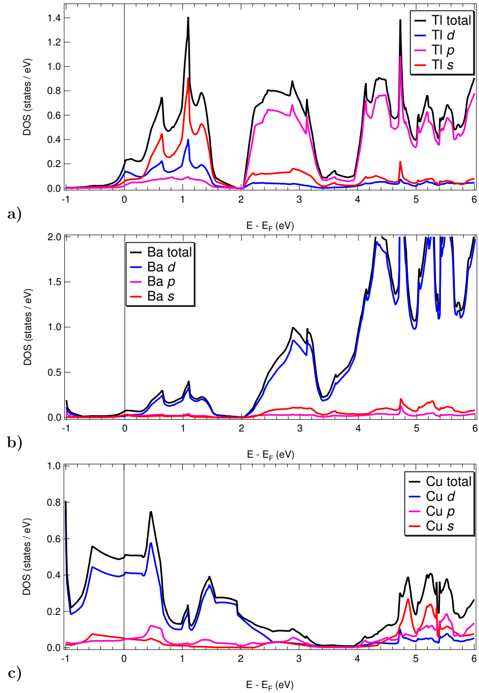
Figure 5.15: Densities of states at and above the Fermi level for a) thallium, b) barium and c) copper, from LDA band structure calculations.
