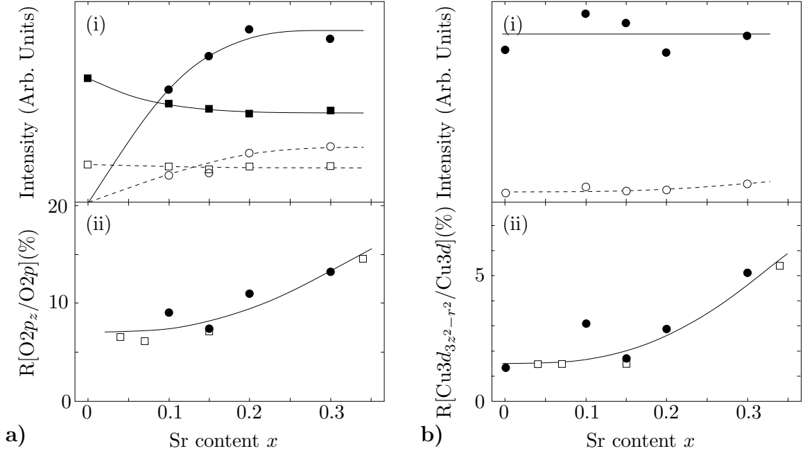
Figure 3.2: Prior to the work reported in this thesis, this constituted all doping-dependent XAS data taken on the overdoped side of the phase diagram (optimal doping is around x=0.18 , but x=0.2 is still quite close to optimal). Adapted from [82]; the material is LSCO, x is the Sr content. a) Oxygen K edge: i) squares are the upper Hubbard band, circles are the valence band, open symbols are 2p_z symmetry, closed symbols are 2p_{x,y} symmetry. ii) Fraction of 2p_z character — open symbols are taken from [83]. b) Cu L\alpha edge: i) closed symbols are 3d_{x^2-y^2} intensity, open symbols are 3d_{3z^2-r^2} symmetry. ii) Fraction of 3d_{3z^2-r^2} character — open symbols are again taken from [83].
