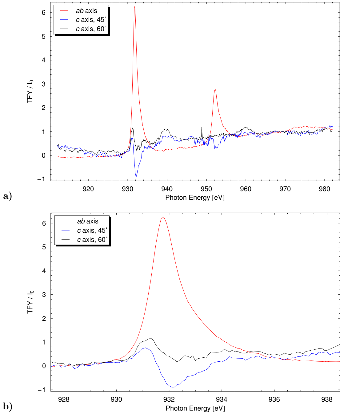
Figure B.8: A comparison of the ab -plane and c -axis Cu L edge spectra for a T_c = 60 K crystal; b) is a detail of the Lα region of a) . The c -axis component is again quite different from the ab component.
