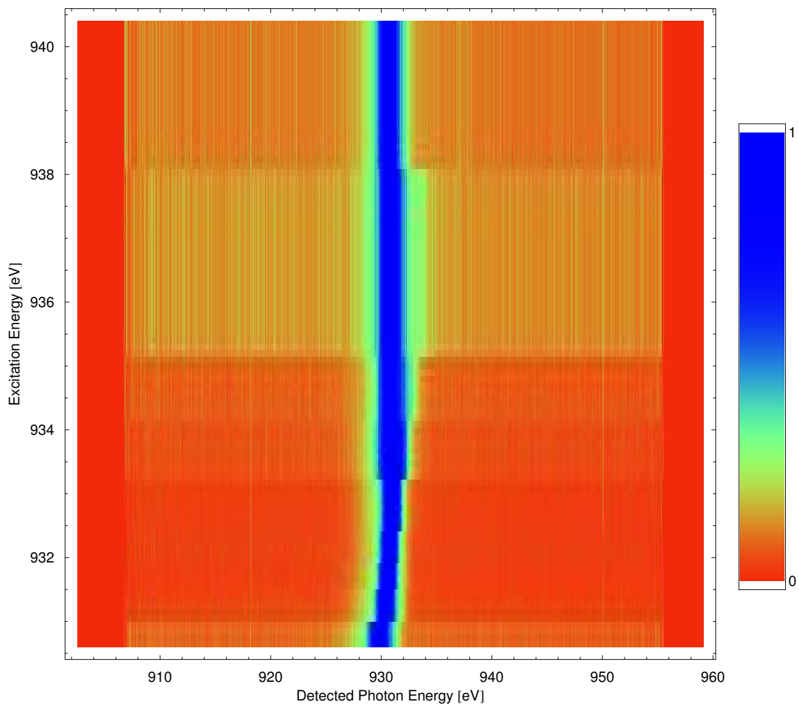
Figure B.18: Copper L edge XES spectra, normalized by peak height, displayed in the form of a density plot.
