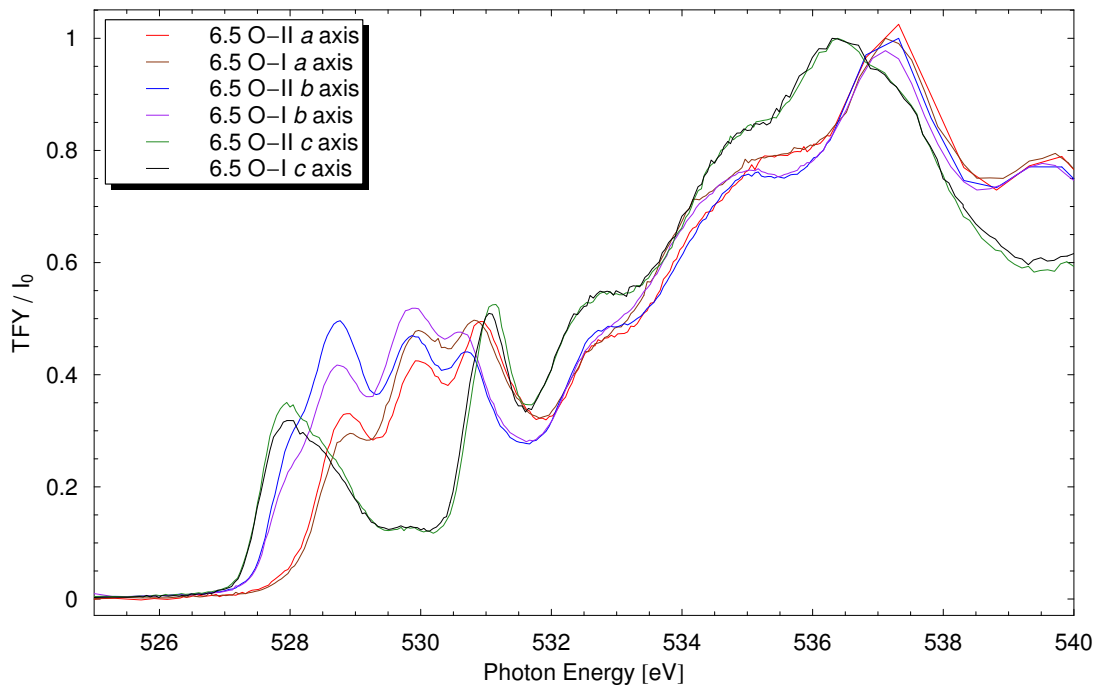
Figure 4.7: Oxygen K edge for Ortho-II ordered and for disordered (Ortho-I) \text{YBa}_2\text{Cu}_3\text{O}_{6.5} crystals. Changes to the prepeaks are clearly visible.
