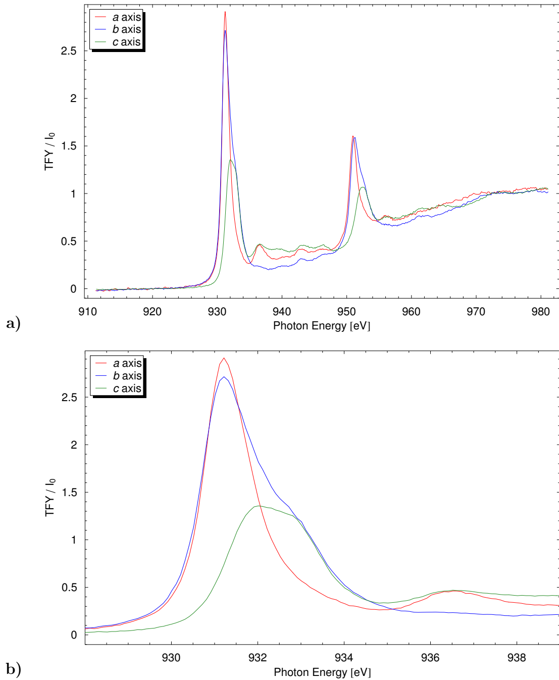
Figure A.3: Copper L edge for YBa 2 Cu 3 O 6.99 crystals as a function of the incident X-ray beam's polarization. a) shows the entire edge, while b) shows the L\alpha edge alone.
