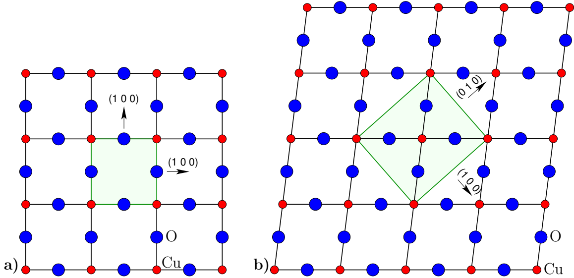
Figure 1.10: The \text{CuO}_2 plane and its slice through the unit cell (in green) are shown for the a) tetragonal phase and the b) orthorhombic phase. The orthorhombic distortion is exaggerated for clarity.
