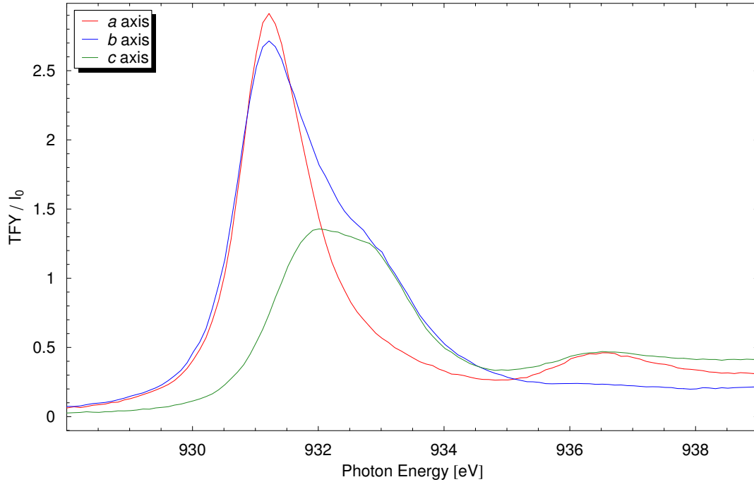
Figure 4.3: Copper L\alpha edge for YBa_2Cu_3O_{6.99} crystals as a function of the incident X-ray beam's polarization.
