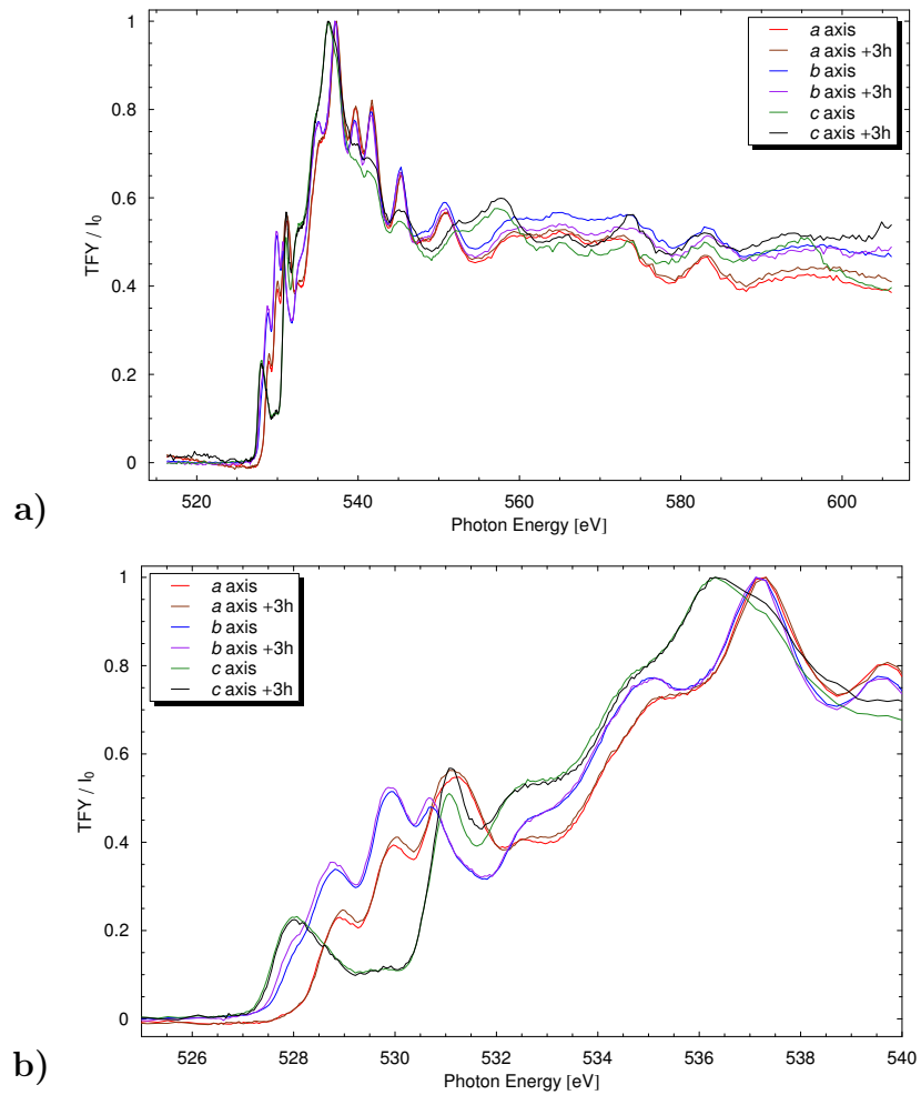
Figure A.6: Oxygen K edge for YBa 2 Cu 3 O 6.35 crystals: a) Entire spectrum, and b) the O K edge and prepeaks.
