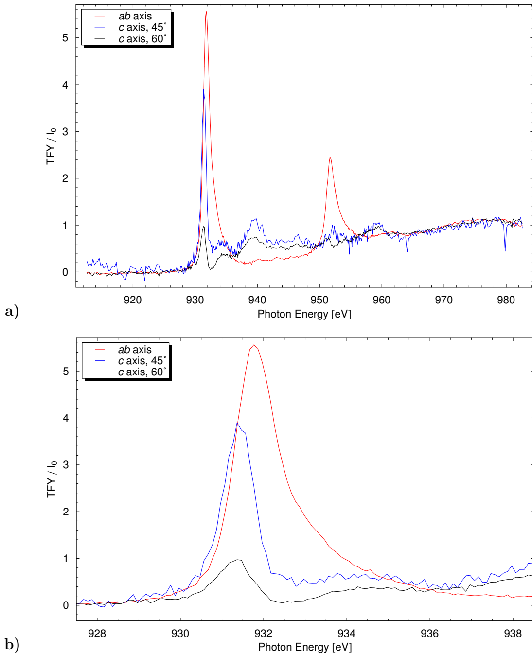
Figure B.12: A comparison of the ab -plane and c -axis Cu L edge spectra for a T_c = 69 K crystal; b) is a detail of the Lα region of a).
