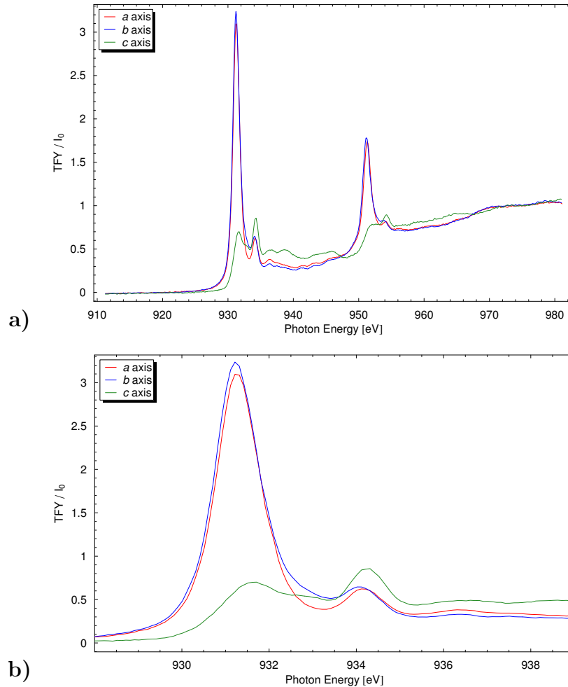
Figure A.5: Copper L edge for YBa 2 Cu 3 O 6.35 crystals: a) Entire spectrum, and b) detail of the Cu L\alpha peak.
