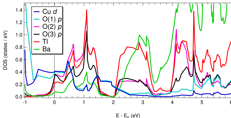
Figure 5.14: Densities of states at and above the Fermi level for the various atomic species and sites, from LDA band structure calculations.
