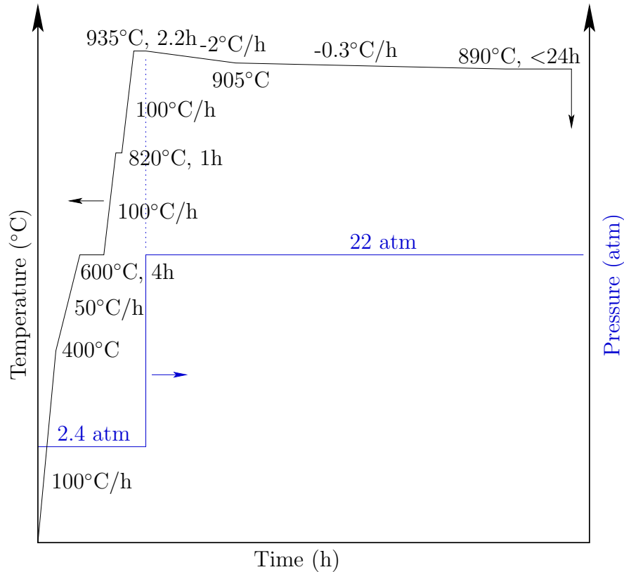
Figure 2.4: Temperature and pressure programs for crystal growth. Shortly before the system begins to cool freely back to room temperature, the rams and crucible are rotated by 180°. Pressures are calculated for the rim, assuming that 1/3 atm is consumed balancing the thallium oxide's vapour pressure. An oxygen overpressure inside the crucible would significantly reduce these numbers.
