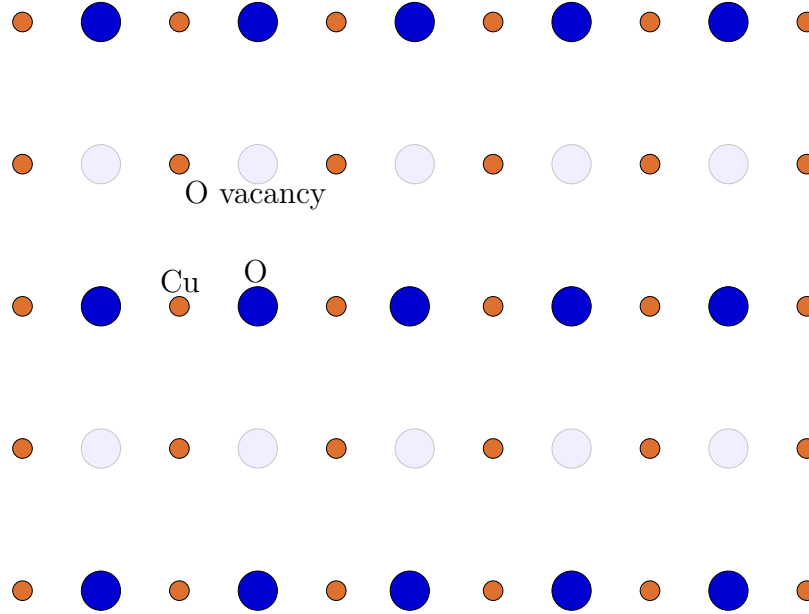
Figure 4.2: Oxygen chain order in Ortho-II \text{YBa}_2\text{Cu}_3\text{O}_{6.50} — full and empty chains alternate.
