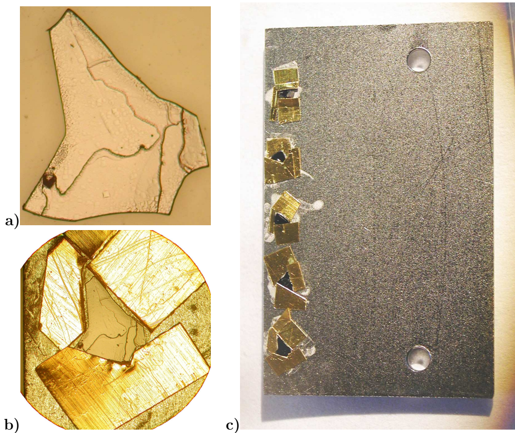
Figure 3.7: A T_c = 9.5 K Tl-2201 crystal and XAS sample plate. a) The T_c = 9.5 K Tl-2201 crystal most thoroughly studied by XAS, after etching but before mounting. Square etch pits are visible, indicating the orientation of the crystal axes. b) The same crystal is shown, attached to the sample plate with silver paint and masked off with gold foil. c) An XAS sample plate with five Tl-2201 crystals mounted on it, including the one shown in the other two panes. From top to bottom, their T_c s are 46 K, 69 K, 69 K, 9.5 K, and 9.5 K. For scale, the sample plate measures \frac{5}{8} " \times 1".
